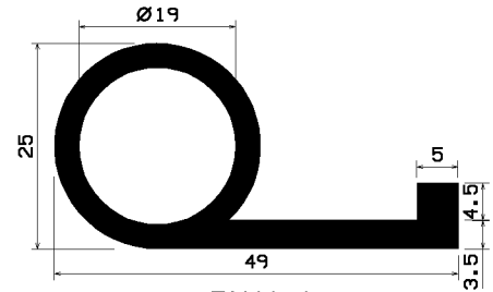
FN1151 EP/s/ 3804
