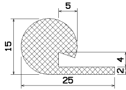
25472 EP/g/ 4267
