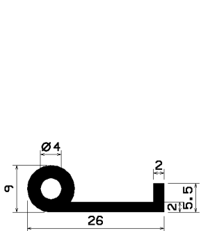
FN2307 FPM/s/ 8063
