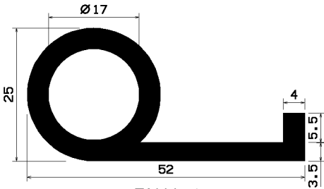
FN1149 EP/s/ 3799
