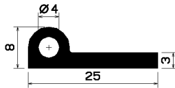
FN1596 Si/rb/ 5294
