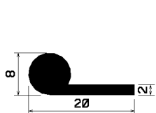
FN2090 Si/I/ 7244
