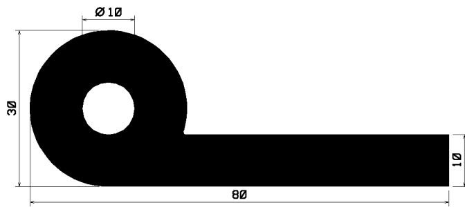
FN2253 FPM/s/7863
