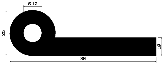
FN2209 EP/s/ 7695
