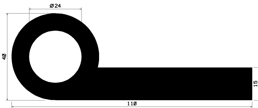
FN2229 EP/s/ 7821
