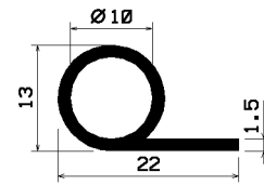
FN1730 Si/rb/ 5935
