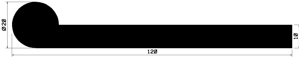
FN2334 EP/s/ 8113
